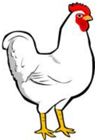
why
